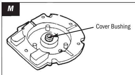
Apply Aquashield® to cover bushing
